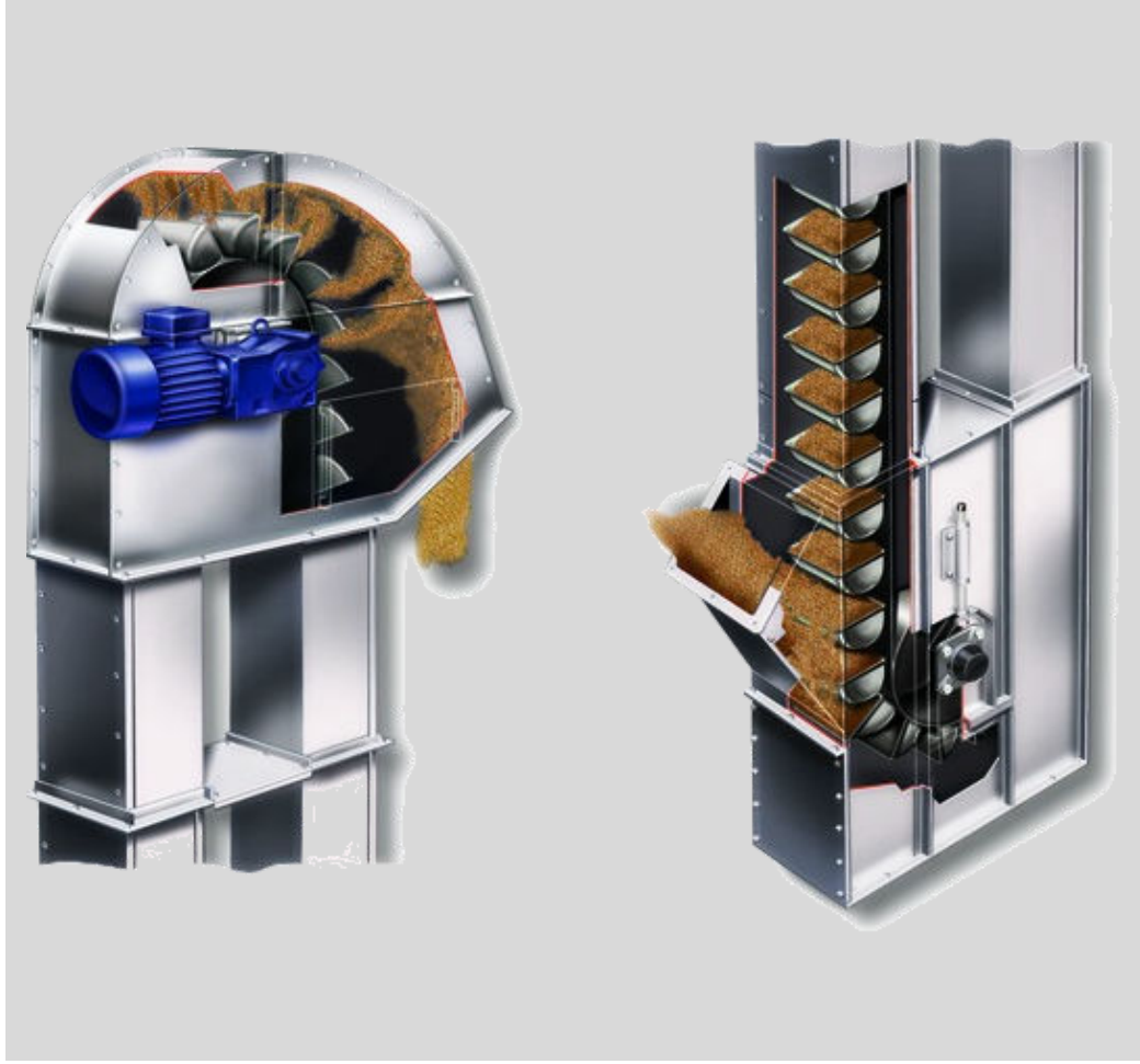
BUCKET ELEVATORS
